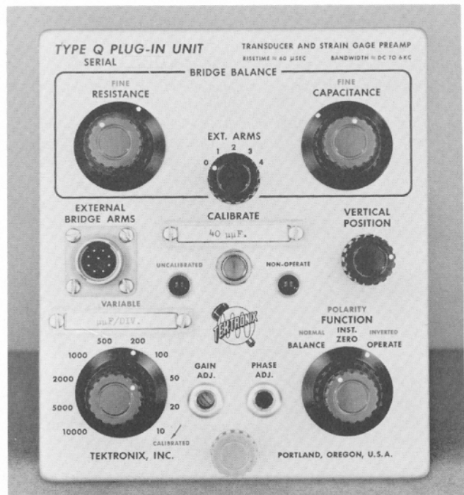
Fig. 2-14. Front panel view of the Type Q Plug-In Unit. The 400 \mu STRAIN and \mu STRAIN/DIV. front panel markings have been changed to 40 \mu\text{f} . and \mu\mu\text{f}/\text{DIV} . respectively by means of small tags placed in the small plastic holders. In this case the scale markings of the control must be divided by 10 to obtain the correct scale factors.
