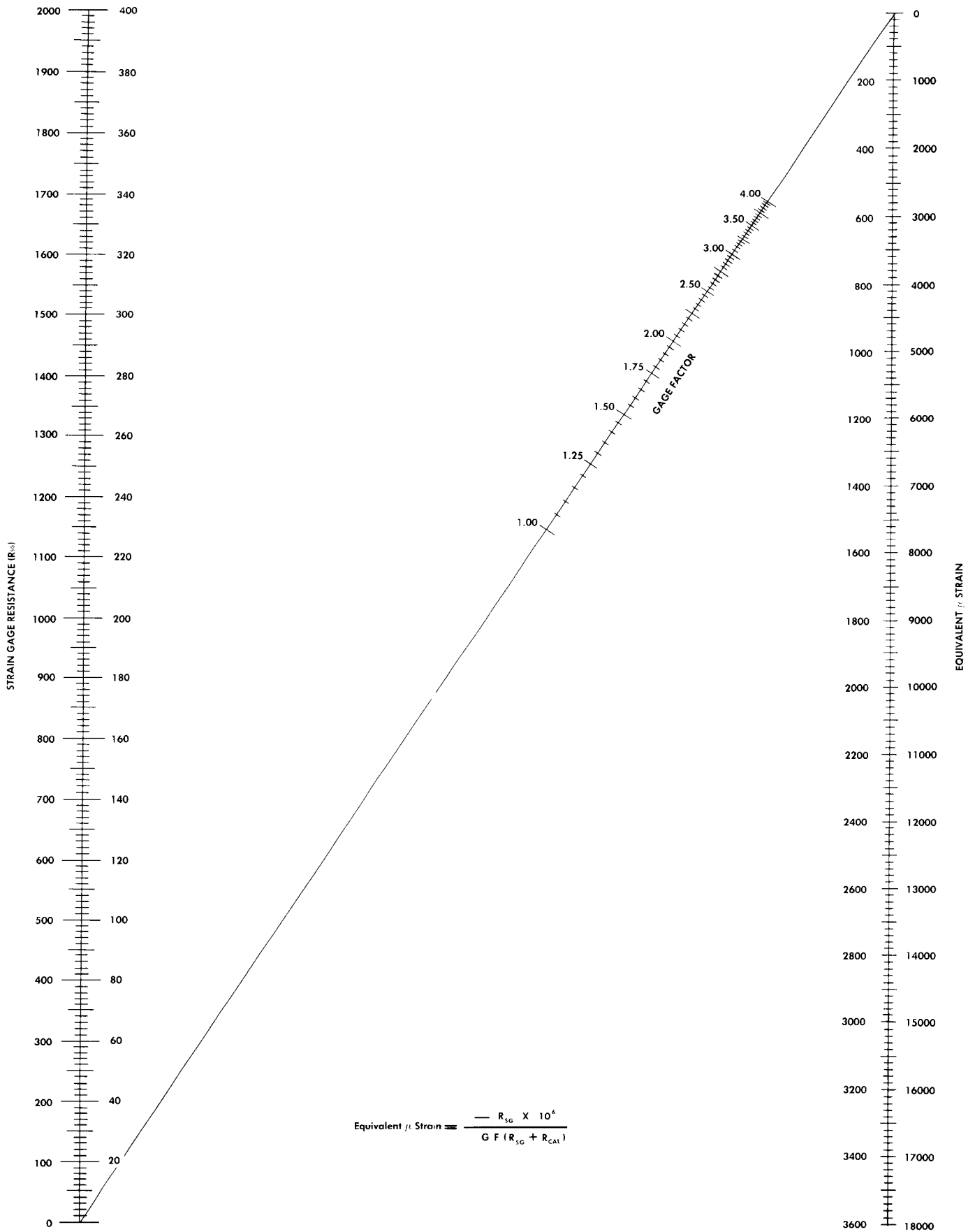
Fig. 2-12. Nomograph for the 150 k calibrator resistor. This nomograph can be used to find the equivalent \mu strain produced by the 150 k calibration resistor when the unit is used with strain gages with various resistances and gage factors.
